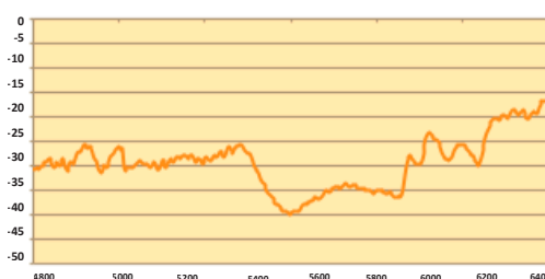
Antenna Cross Polarity 4800-6400 MHz
