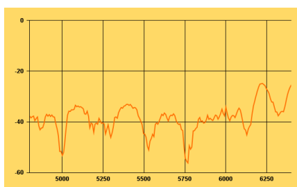
Antenna Port to Port Isolation 4800-6400 MHz
