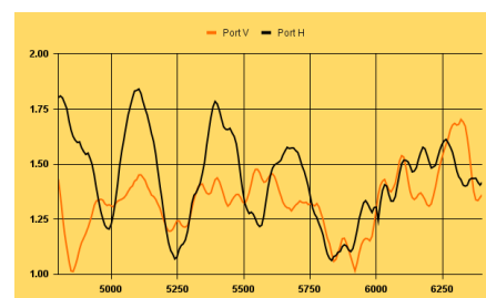
Antenna VSWR 4800-6400 MHz
