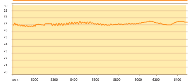
Antenna Gain 4800-6400 MHz
